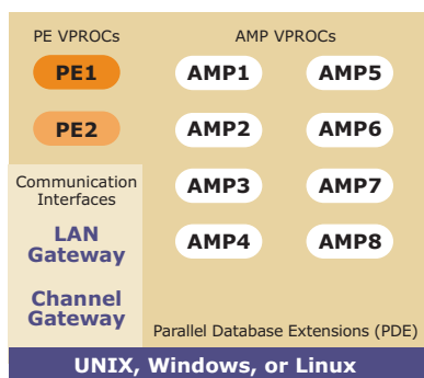
Figure 2. Teradata Node SW Architecture.
